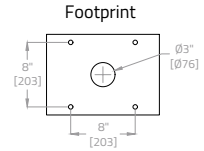
STD WSB Bottom Plate 1/2" [6.4] Steel Plate
